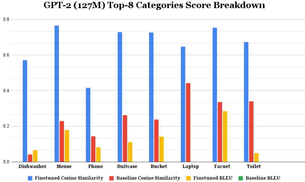
Figure 3: Top 8 Categories Comparison. We compare the cosine similarity and BLEU scores for the Top-8 Categories. Note that the BLEU score for the baseline is so low, that it is not visible in this chart.
